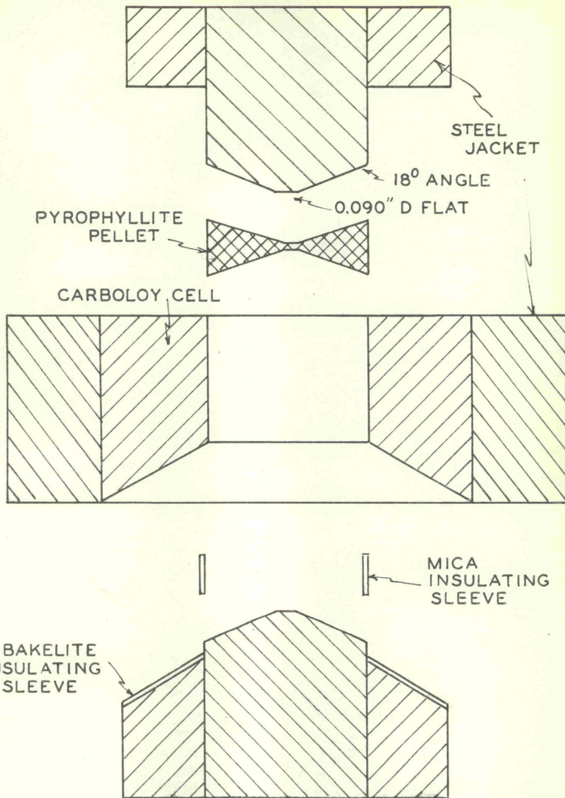
FIG. 1 RESISTANCE CELL-OVERALL SCHEMATIC DRAWING
